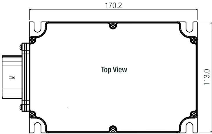
Dimension Drawing (mm)
