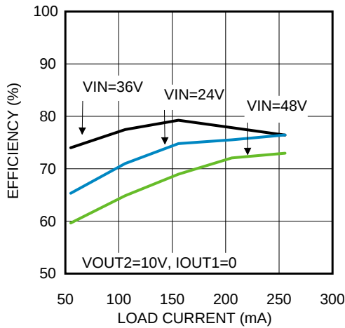
Figure 1. Efficiency at 750 kHz, V_{OUT1} = 10 V
