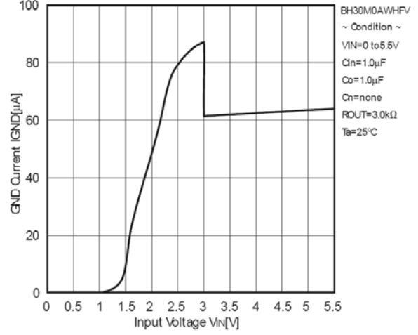
Figure 4. GND Current vs. Input Voltage
