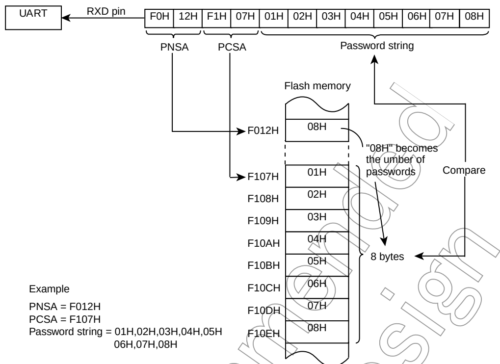
Figure 15-5 Password Comparison
