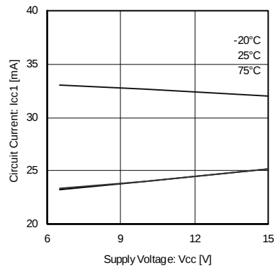
Fig.5 Supply current 1 (forward) (BA6285FS)
