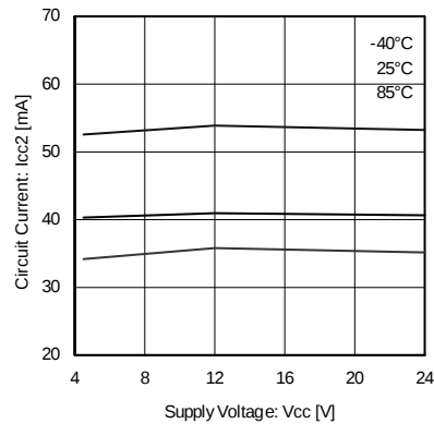
Fig.8 Supply current 2 (brake) (BA6285AFP-Y)
