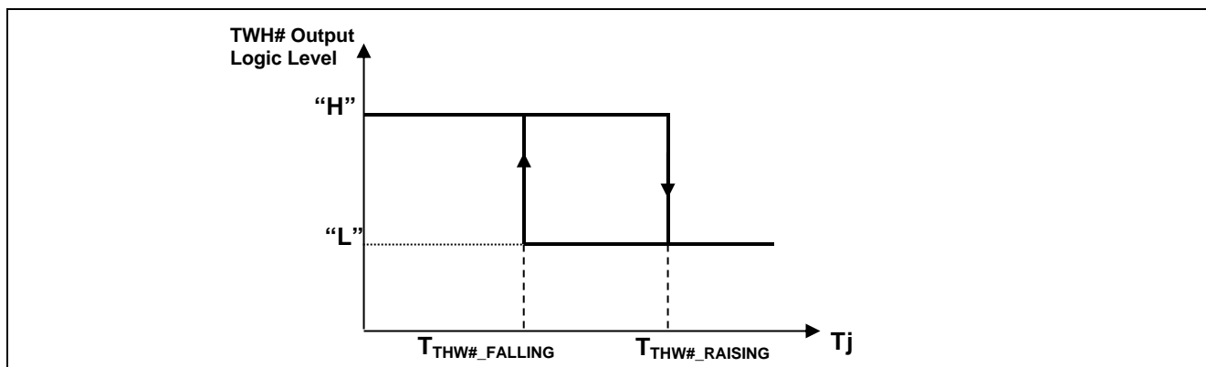
Figure 6 Thermal warning
