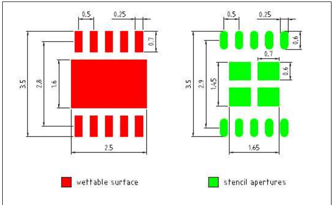
Figure 10 Footprint
