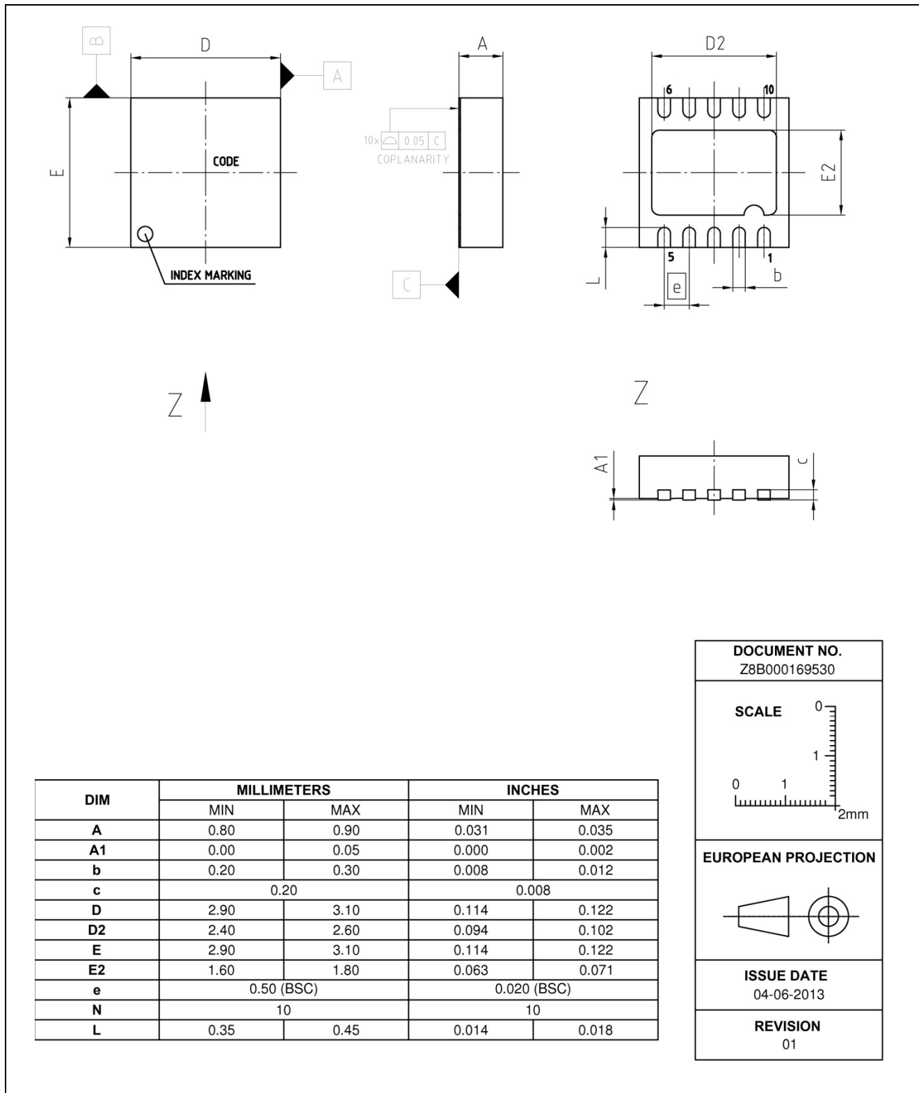
Figure 9 Mechanical dimensions
