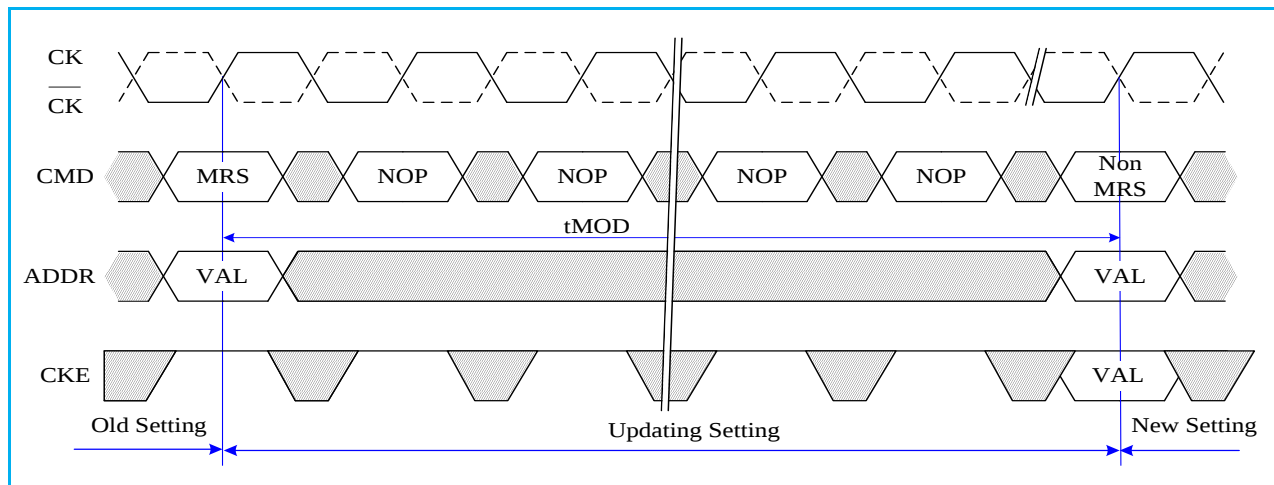
Fig. 7: t_{MOD} Timing
