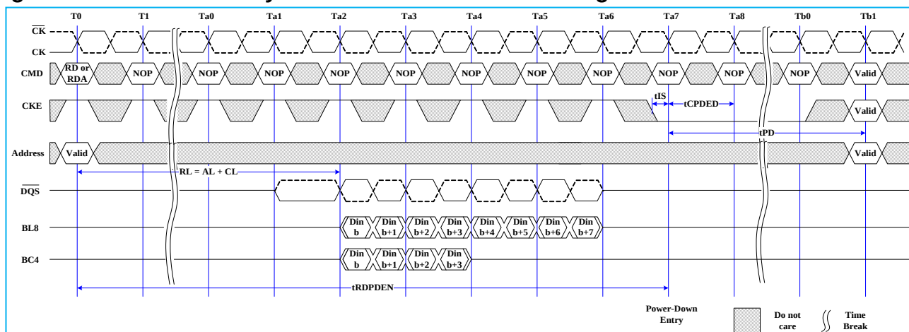
Fig. 38: Power-Down Entry after Write with Auto Precharge
