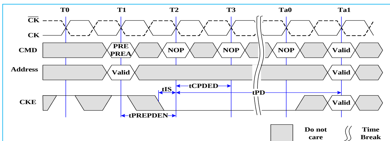
Fig. 44: Precharge/Precharge all Command to Power-Down Entry
