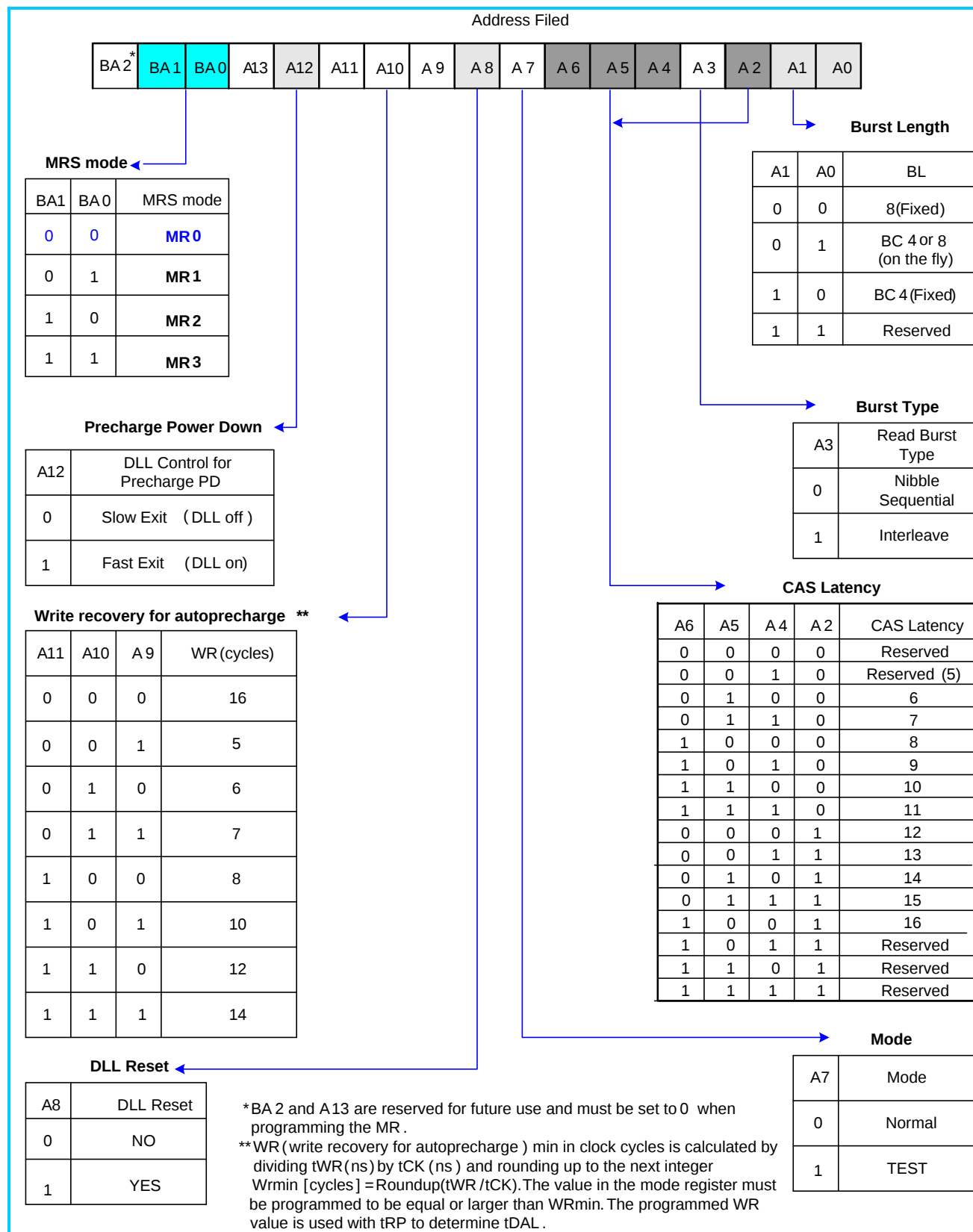
Fig. 8:MR0 Definition
