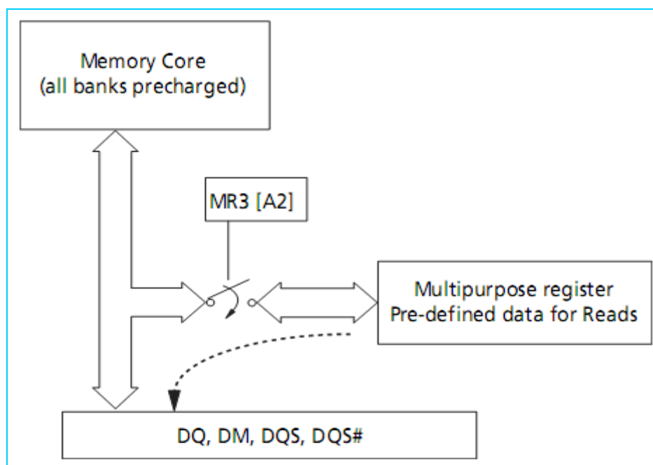
Fig. 12: MPR Block Diagram
