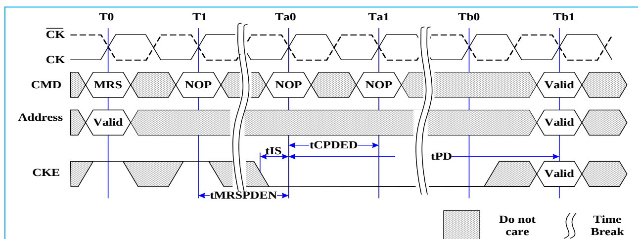
Fig. 45: MRS Command to Power-Down Entry
