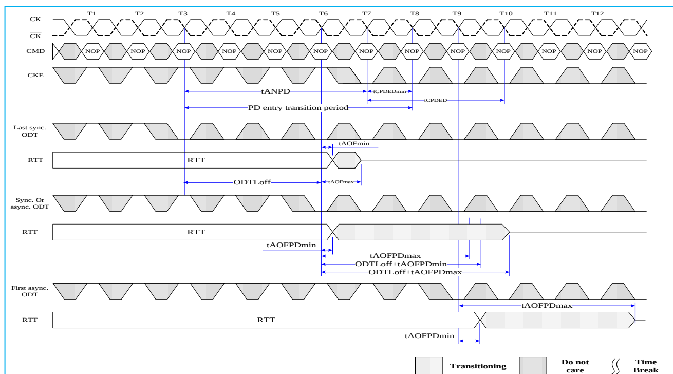
Fig. 56: Synchronous to asynchronous transition during Precharge Power Down (with DLL frozen) entry (AL=0; CWL=5; tANPD=WL-1=4)
