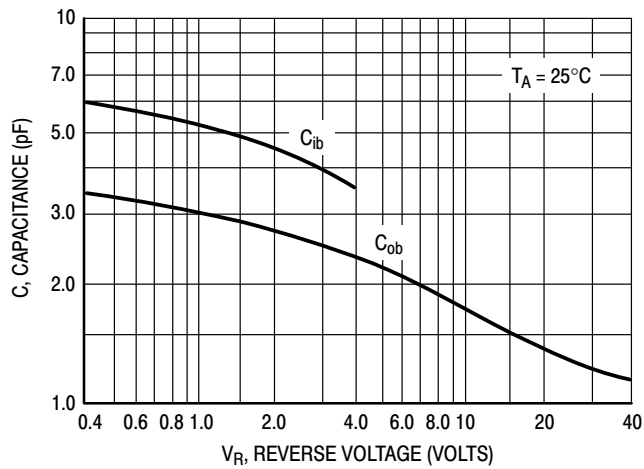
Figure 39. Capacitances
