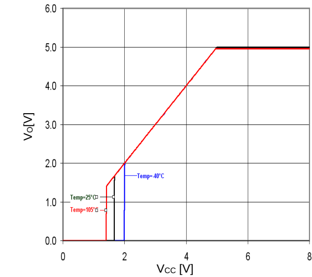
Fig.27 V_{cc} - V_o ( I_o=0mA )
