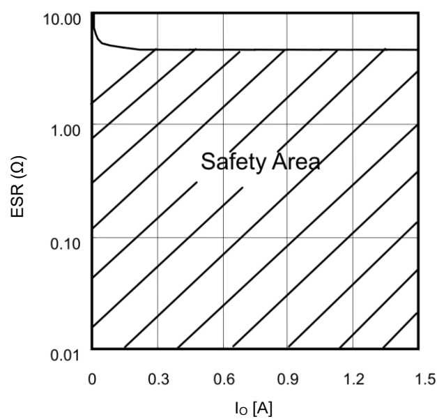
Fig.31 Operation Safety area
