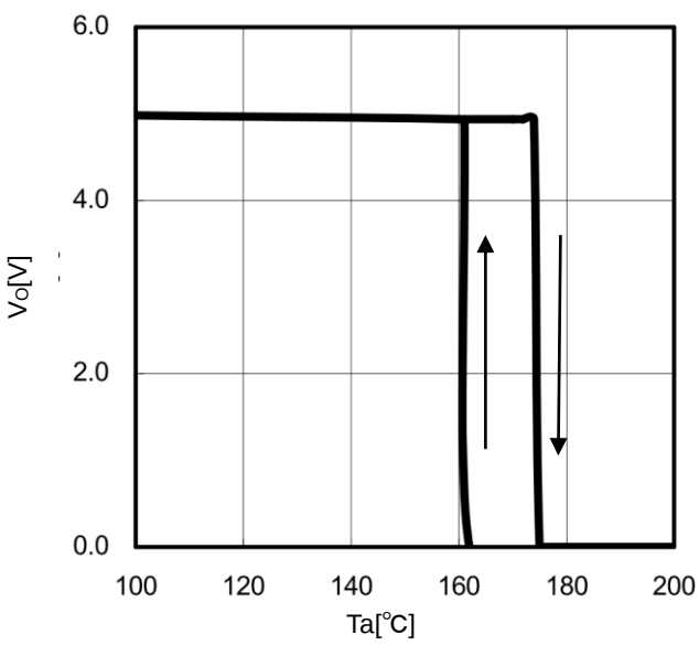
Fig.28 TSD ( I_o=0mA )
