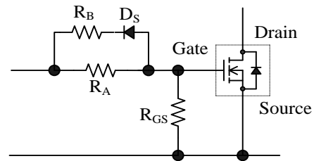
Figure 9-1. Power MOSFET Peripheral Circuit
