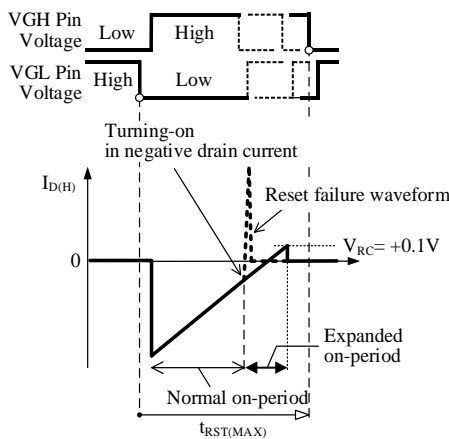
Figure 8-31. Reset Detection Operation Example at High-side On Period
