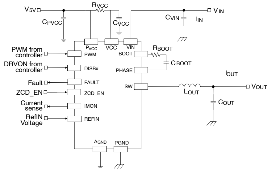
Figure 1. Application Diagram
