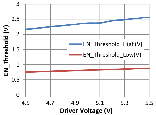
Figure 17. EN Threshold vs. Driver Voltage
