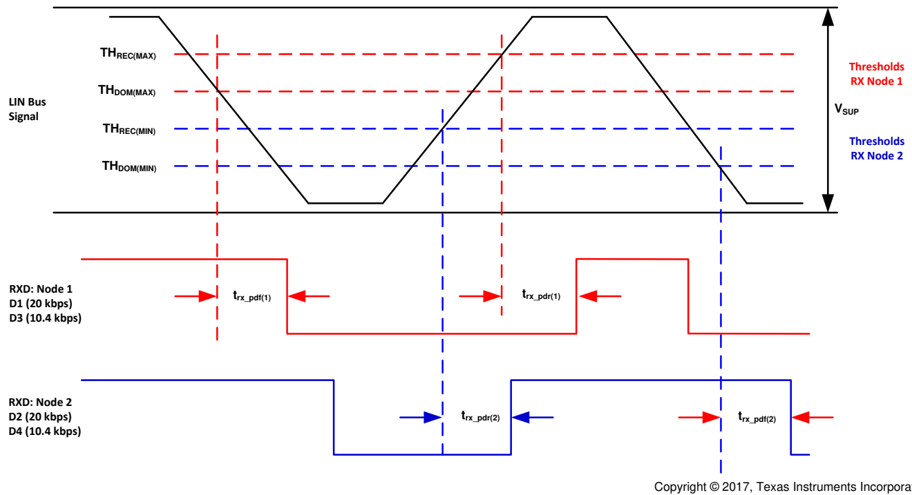
Figure 7-14. Propagation Delay
