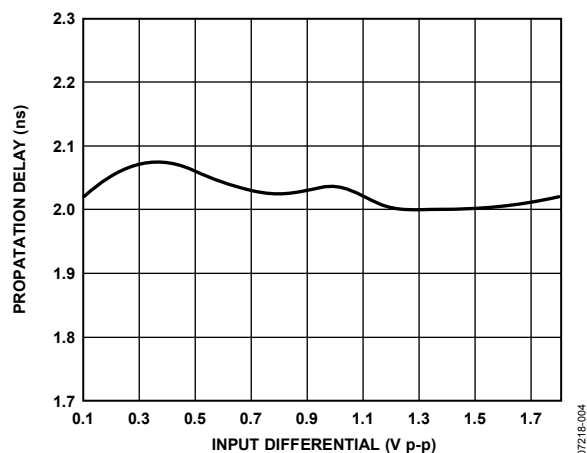
Figure 4. LVDS Propagation Delay vs. Input Differential Voltage ( V_{IP} )
