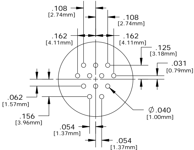
FACE VIEW W4281-12PG-300 12-POS.
