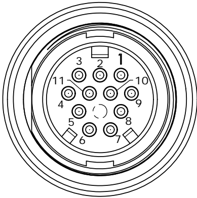
FACE VIEW W4281-11PG-300 11-POS.
