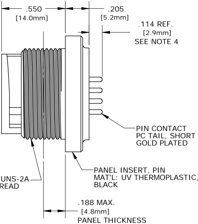
PC TAIL VIEW W4281-10PG-300 - 10-POS. (11&12 CLOSED) W4281-11PG-300 - 11-POS. (12 CLOSED) W4281-12PG-300 - 12-POS. (ALL OPEN)
