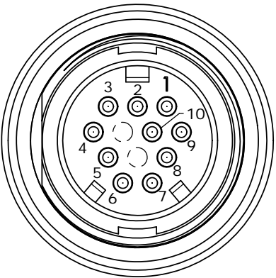
FACE VIEW W4281-10PG-300 10-POS.
