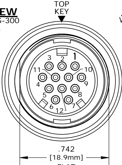
FACE VIEW W4281-12PG-300 12-POS.
