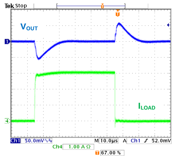
Load Transient: V_{IN} = 3.3V , V_{OUT} = 1.2V
