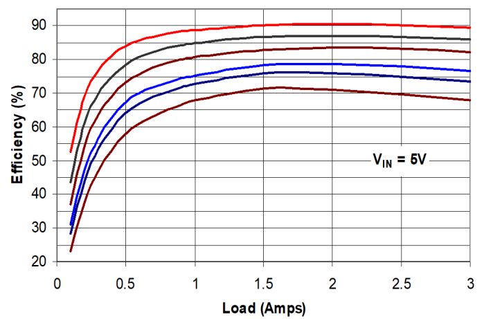
Efficiency V_{IN} = 5.0V V_{OUT} (From top to bottom) = 3.3, 2.5, 1.8, 1.2, 1.0, 0.75V
