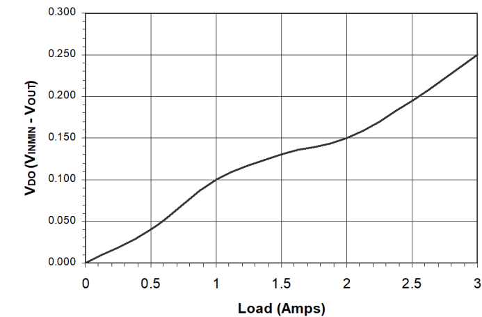
Drop-Out Voltage
