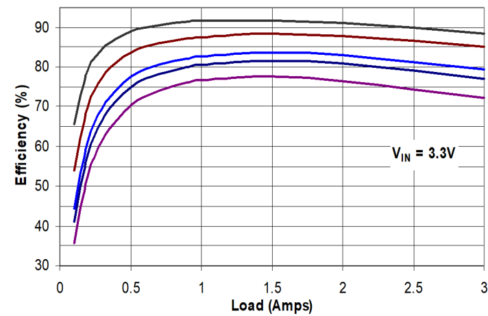
Efficiency V_{IN} = 3.3V V_{OUT} (From top to bottom) = 2.5, 1.8, 1.2, 1.0, 0.75V
