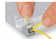
Inserting/removing a conductor via finger-operated lever – 256 Series.
