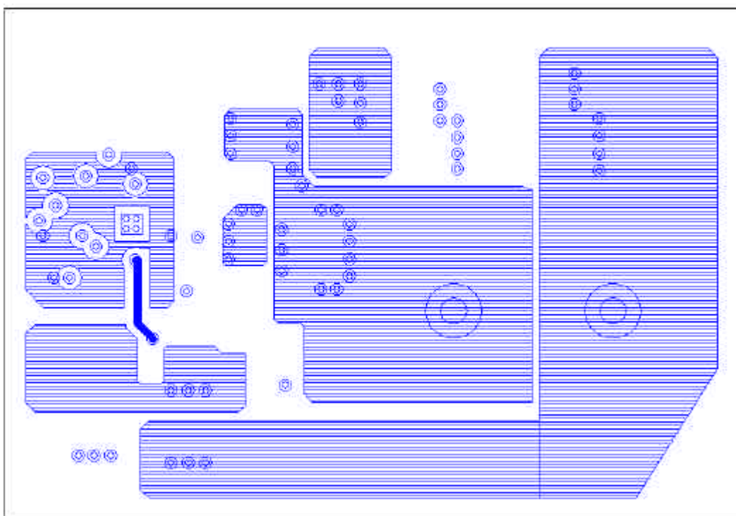
Figure 17 Power layer
