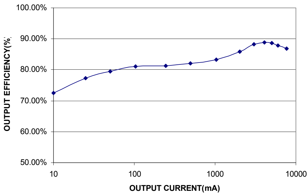
Fig. 10 Output efficiency
