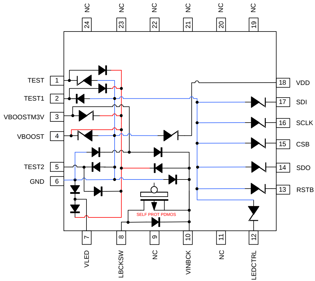
Figure 3. ESD Schematic
