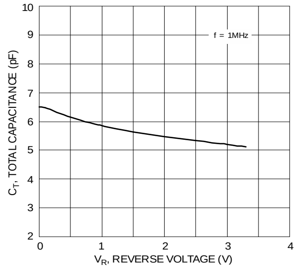
Figure 4 Typical Total Capacitance vs. Reverse Voltage
