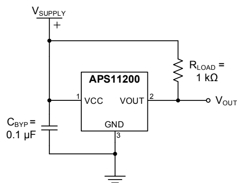
Figure 1: Typical Application Circuit
