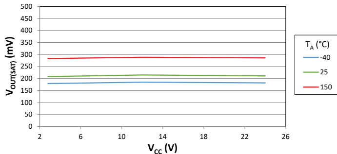
Average Low Output Voltage versus Supply Voltage for I_{OUT} = 20\text{ mA}
