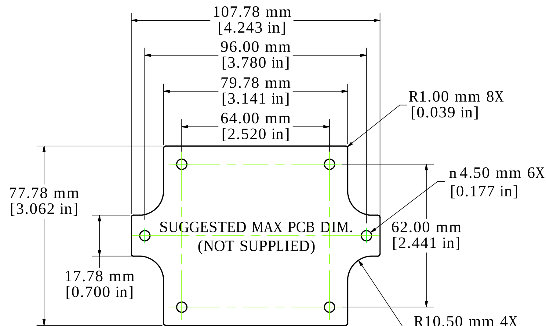
PCB
