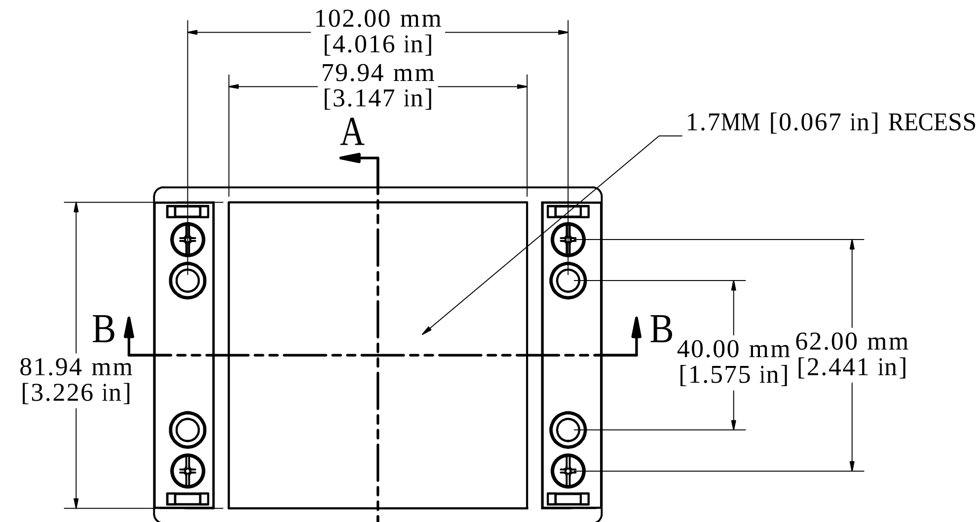
ASSEMBLY - TOP VIEW
