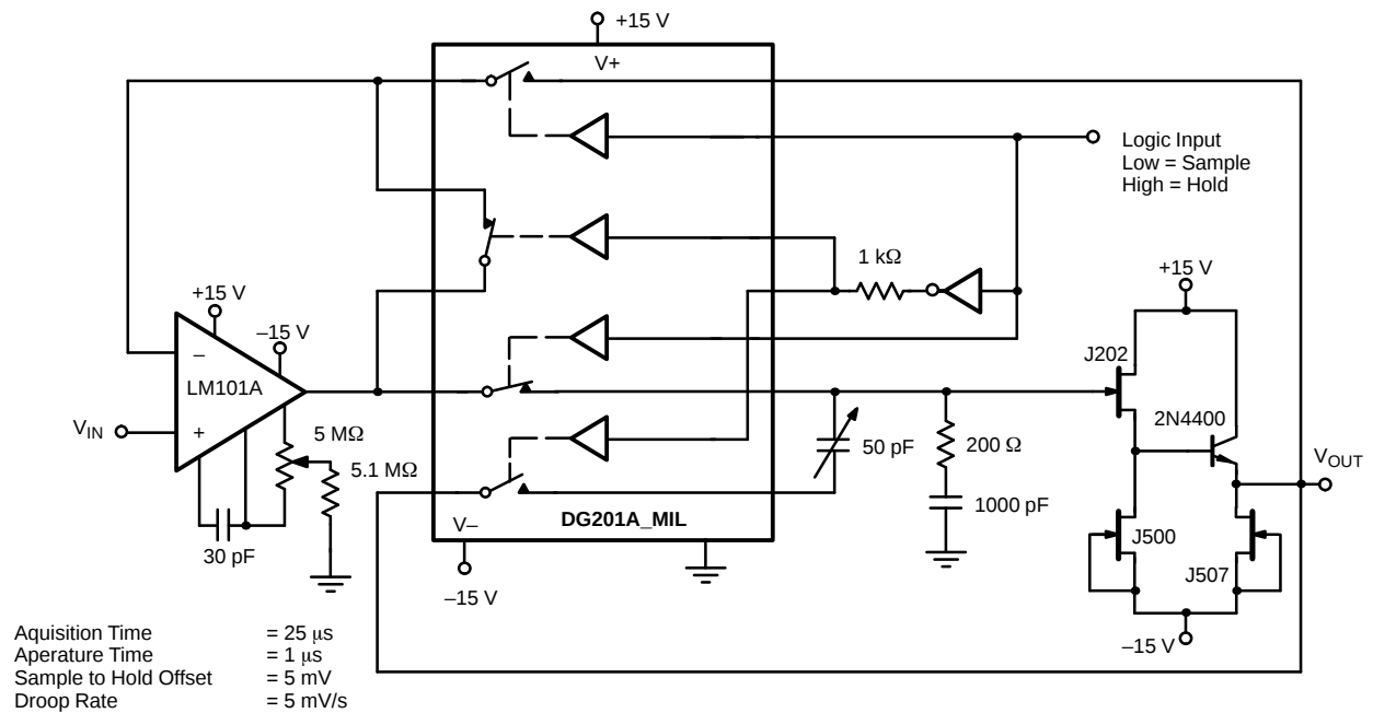
FIGURE 6. Sample-and-Hold
