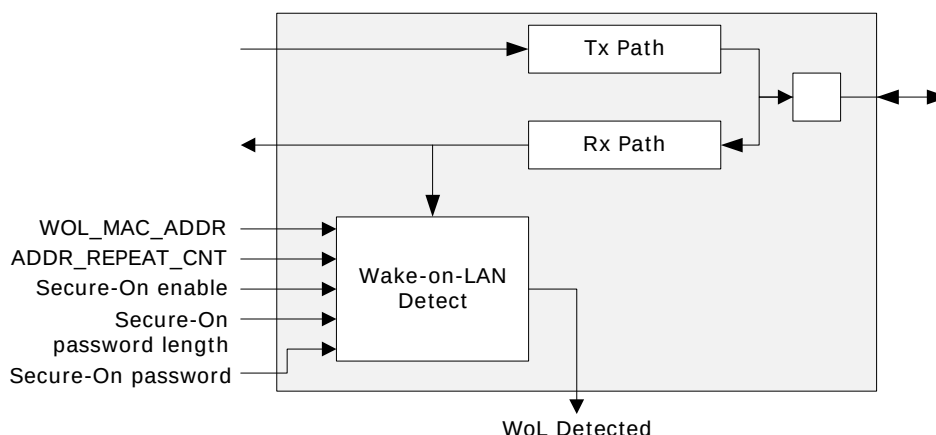
Figure 17 • Wake-on-LAN Functionality
