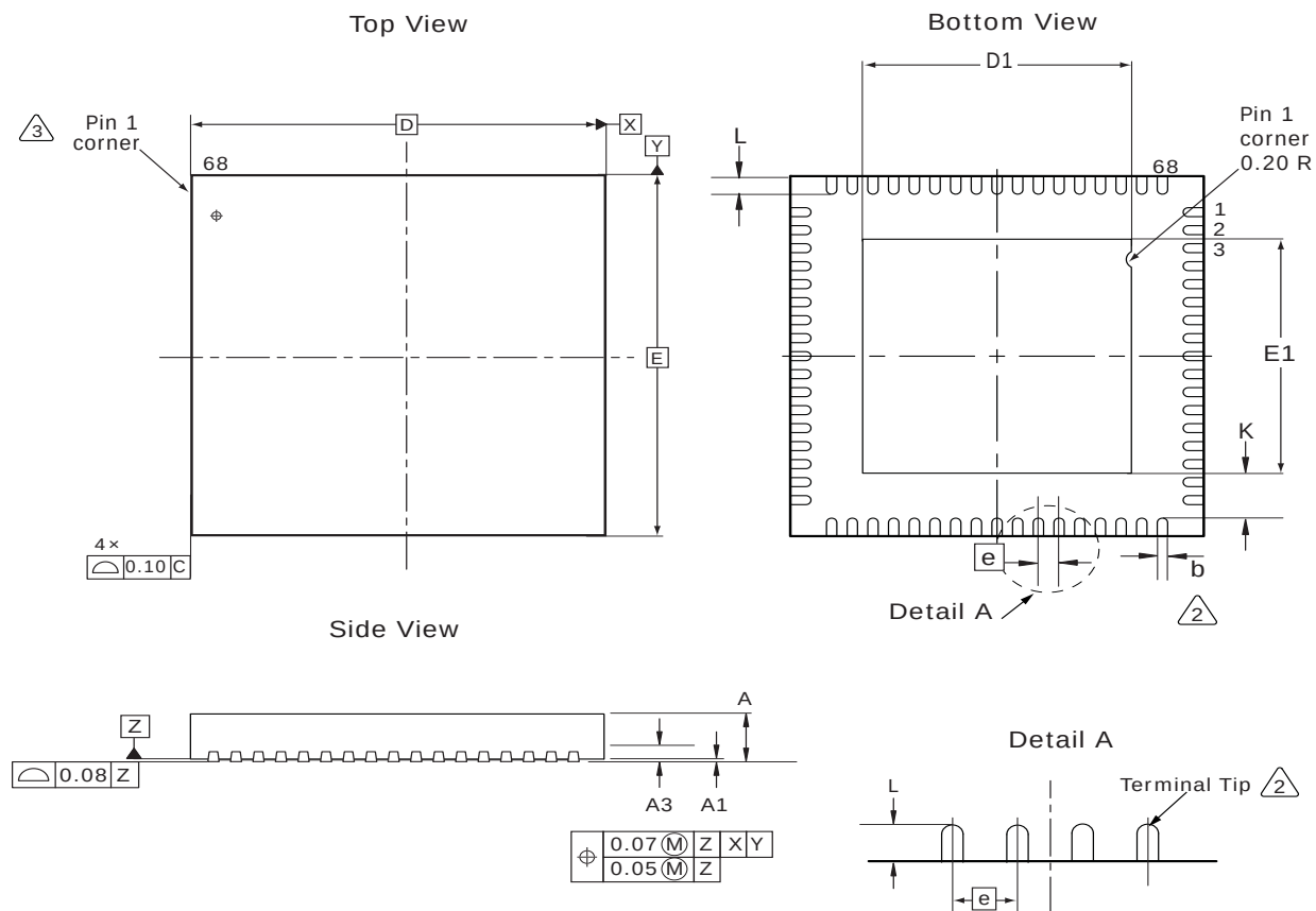
Figure 30 • Package Drawing
