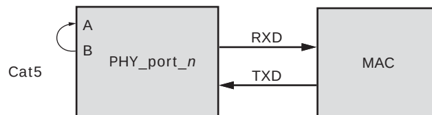
Figure 20 • Connector Loopback Diagram
