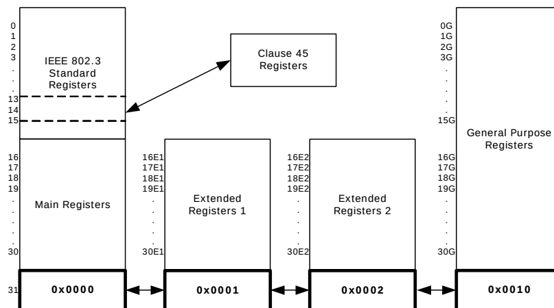
Figure 21 • Register Space Diagram
