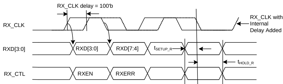
Figure 27 • Compensated Output RGMII Timing
