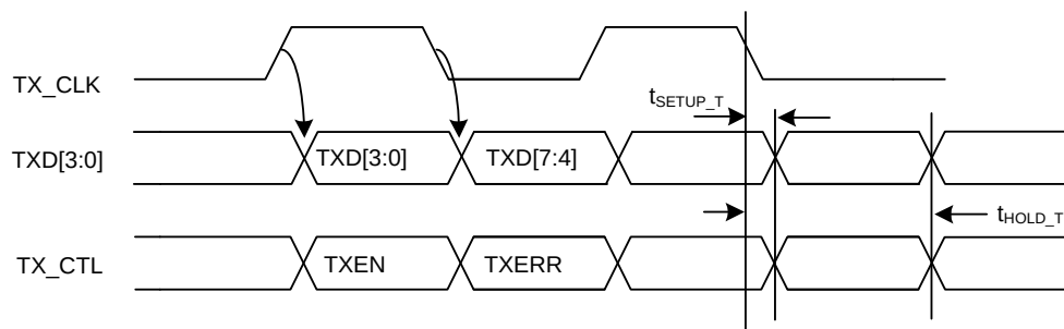
Figure 26 • Compensated Input RGMII Timing
