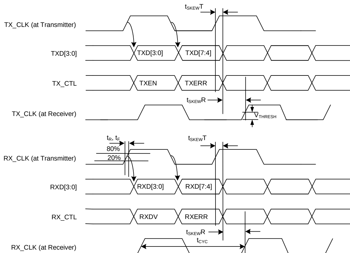
Figure 25 • Uncompensated RGMII Timing
