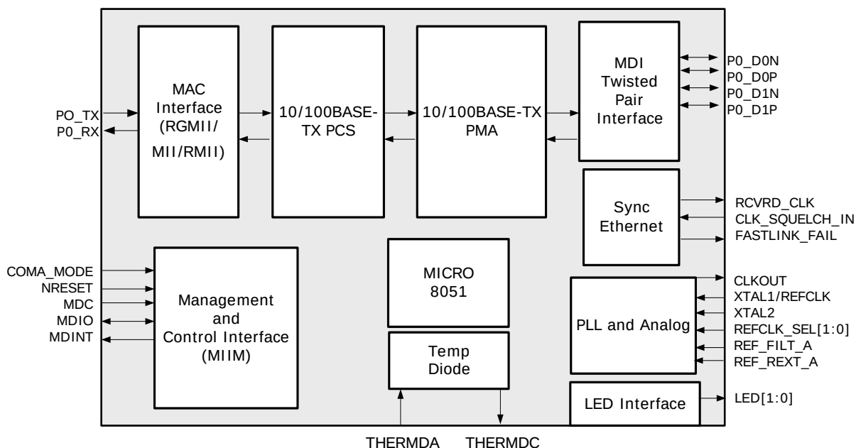
Figure 2 • Block Diagram
