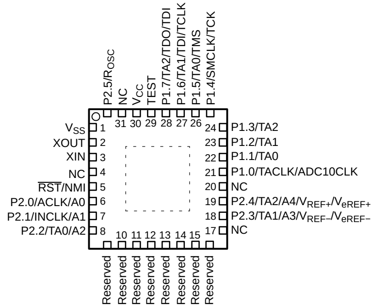
RHB PACKAGE (TOP VIEW)
