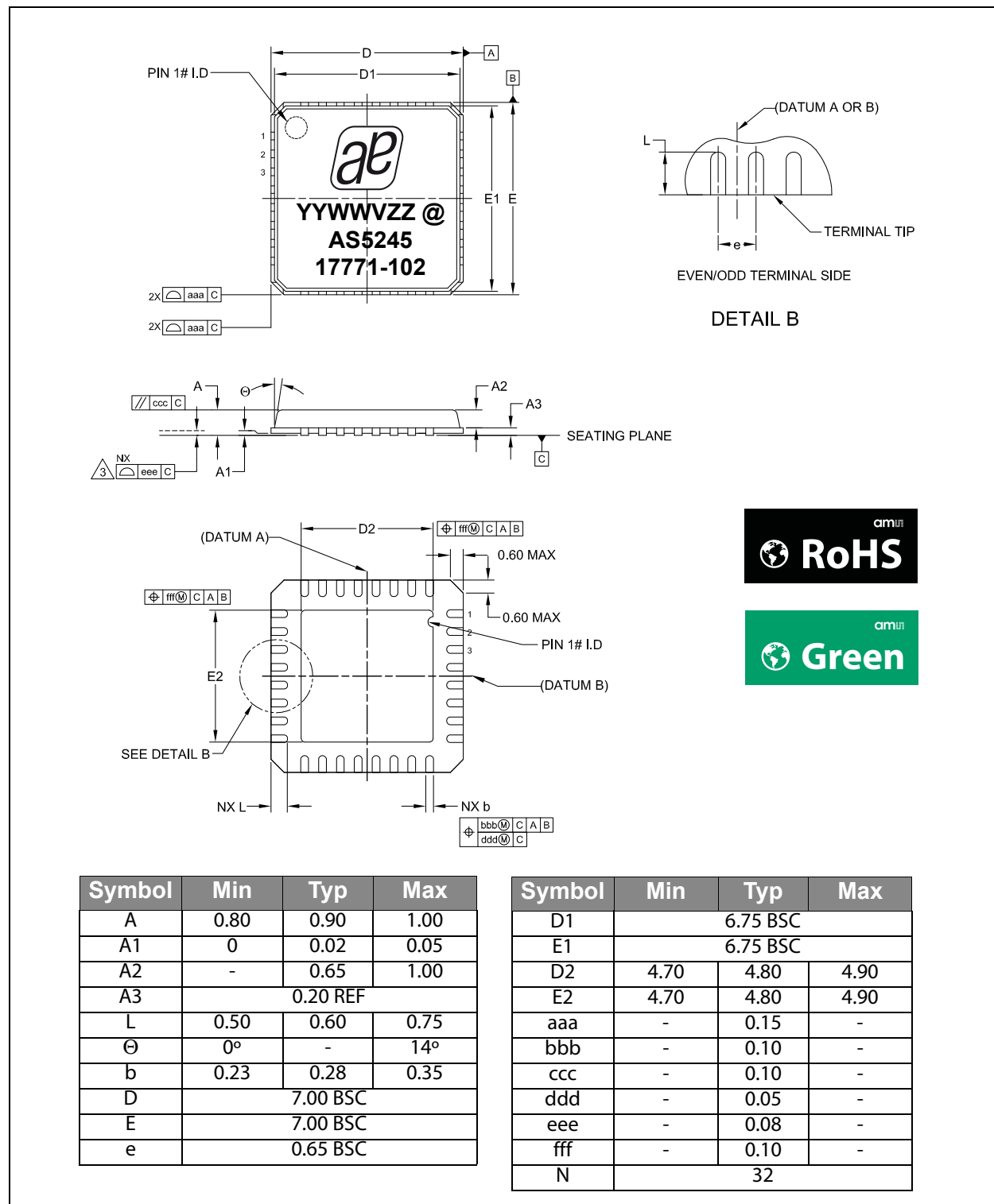
Figure 34: Package Drawing
