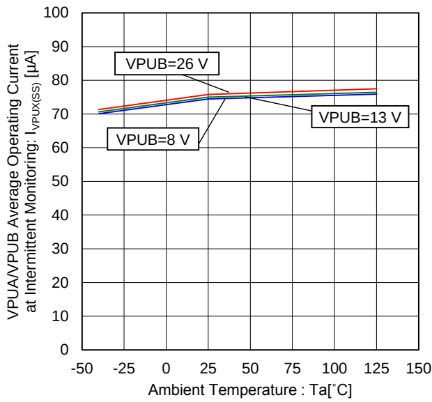
Figure 26. VPUA/VPUB Average Operating Current at Intermittent Monitoring vs Ambient Temperature (Monitoring Period: 50 ms, Strobe Time: 125 \mu s , Source/Sink Current Setting: 1 mA)
