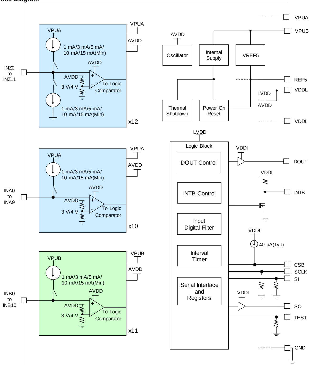
Figure 3. Block Diagram
