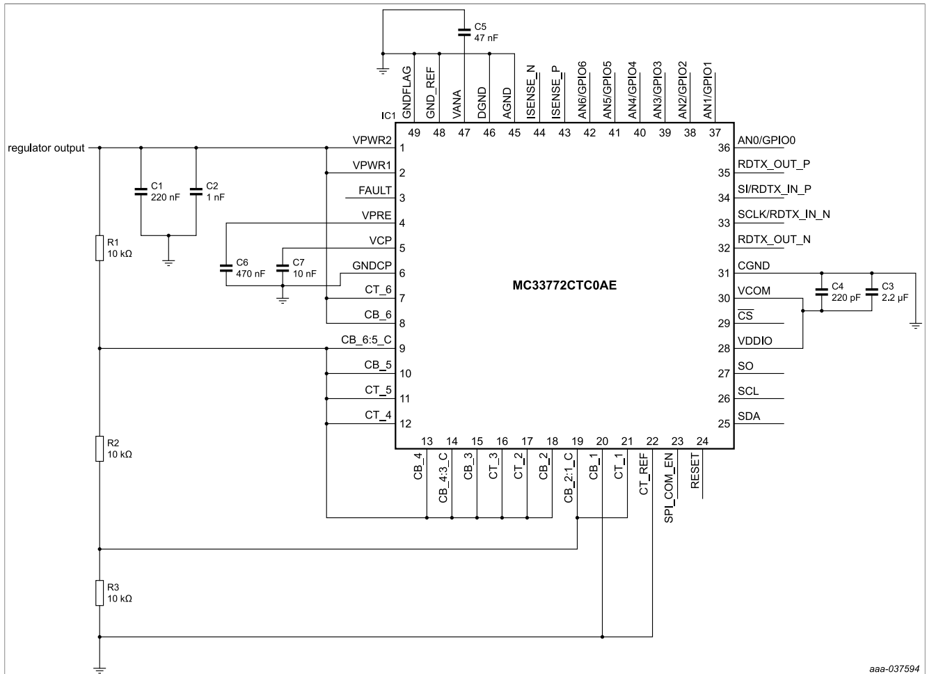
Figure 50. Analog Front End connection
