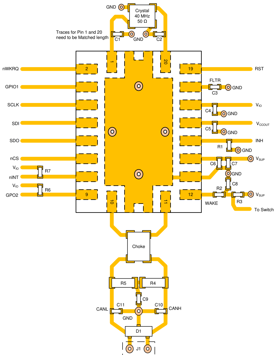
Figure 113. Example Layout
