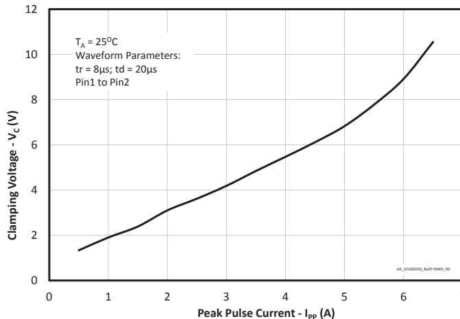
8x20us Clamping Performance Forward
