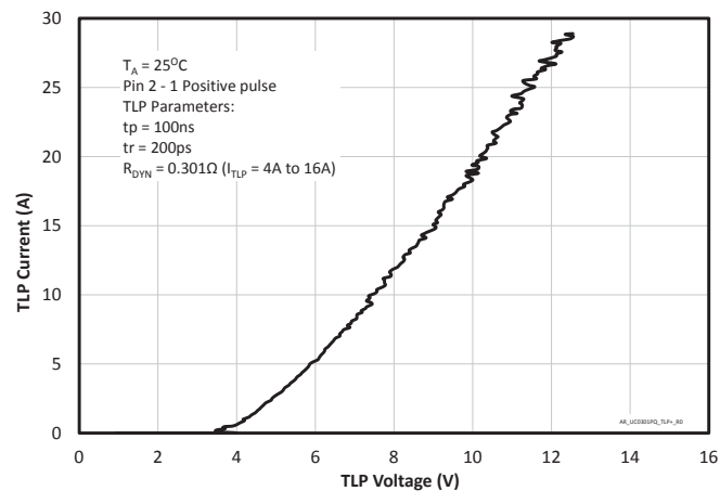
TLP Characteristics Reverse
