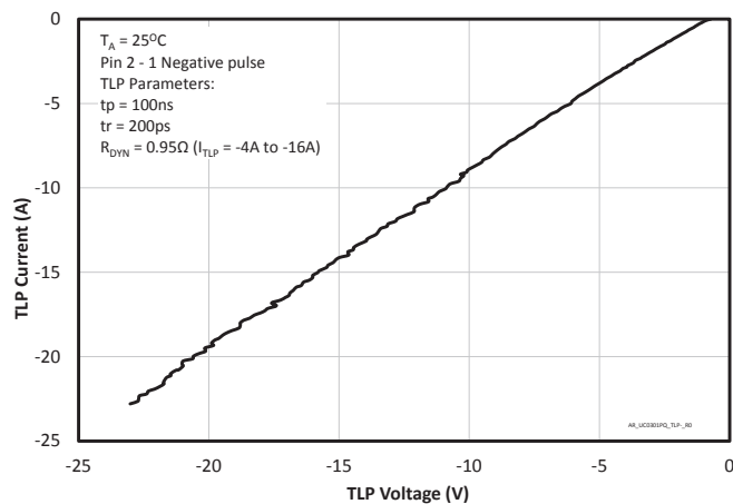
TLP Characteristics Forward
