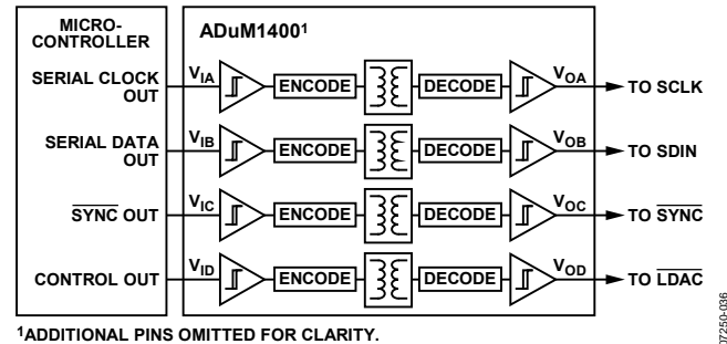
Figure 30. Isolated Interface
