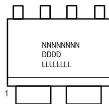
Figure 16: Custom 6-Pin SOIC (Suffix LZ)
