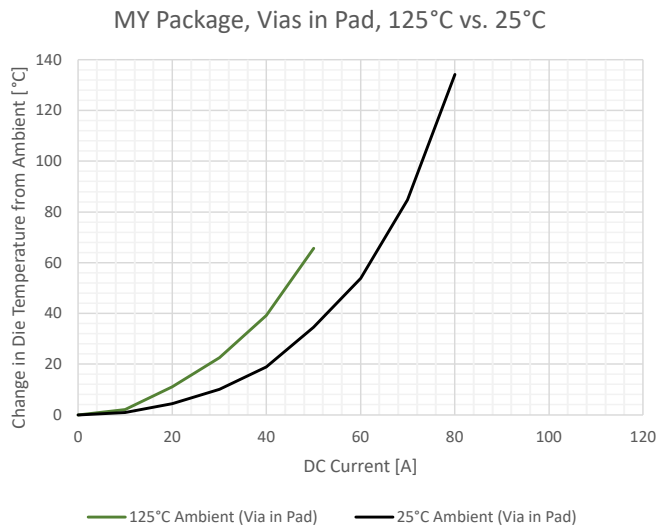
Figure 13: MY Package Comparison at 125°C and 25°C, In-Pad Vias
