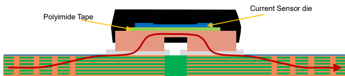
Figure 10: Vias Not Present Under Copper Pads (LZ Package)
