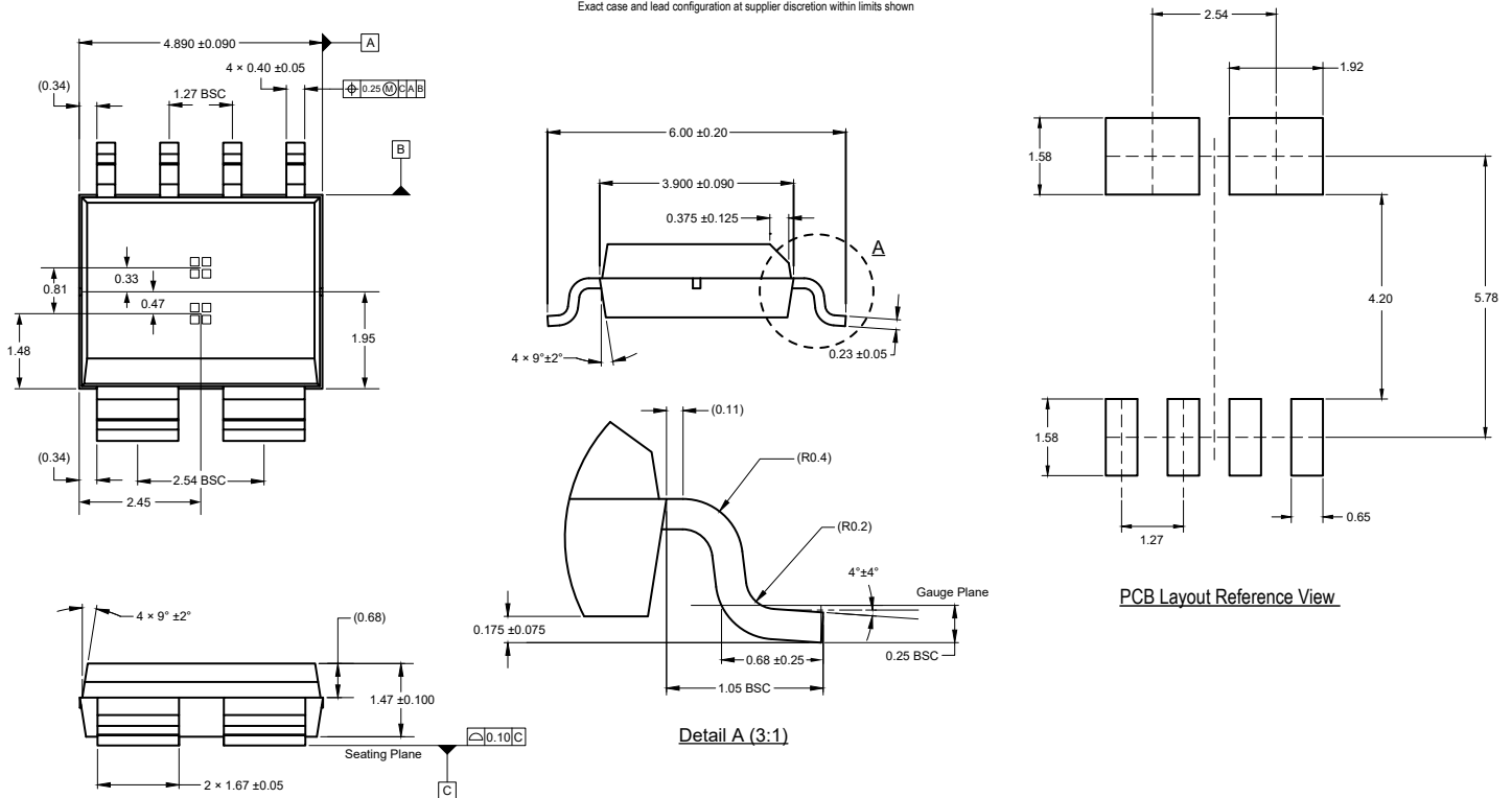
Figure 16: Custom 6-Pin SOIC (Suffix LZ)
