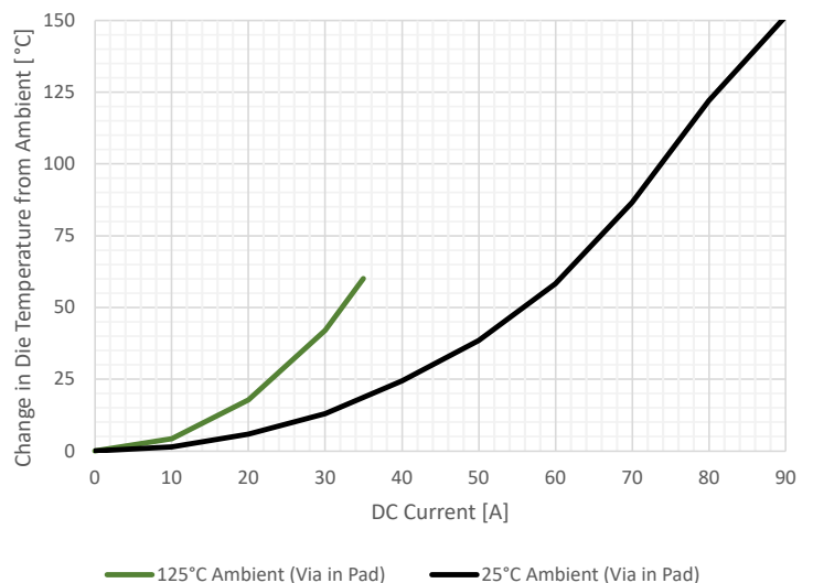
Figure 12: LZ Package Comparison at 125°C and 25°C, In-Pad Vias
