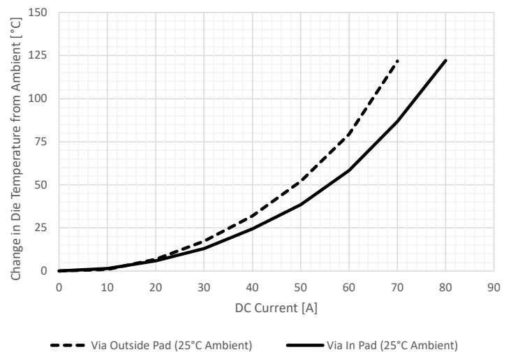
Figure 11: LZ Package Comparison with and without In-Pad Vias at Ambient Temperature
