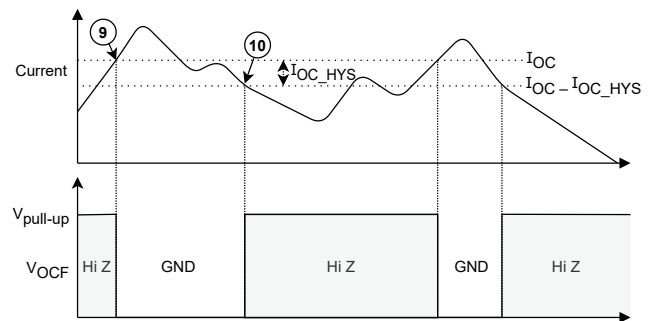
Figure 7: Fault Thresholds and OCF Pin Functionality
