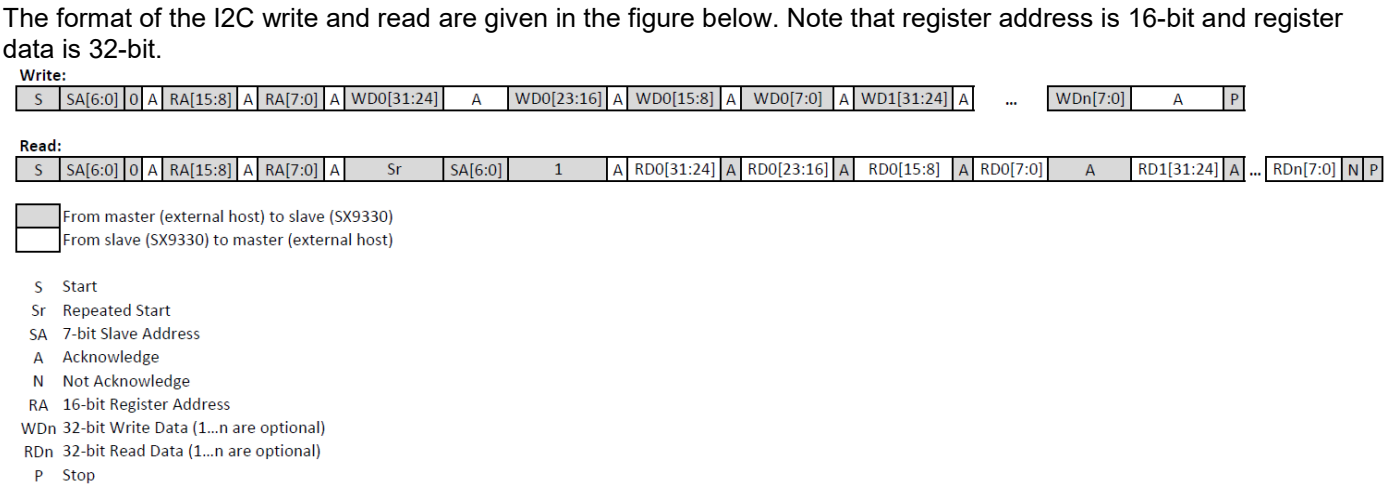
Figure 20: I2C Read/Write Format
