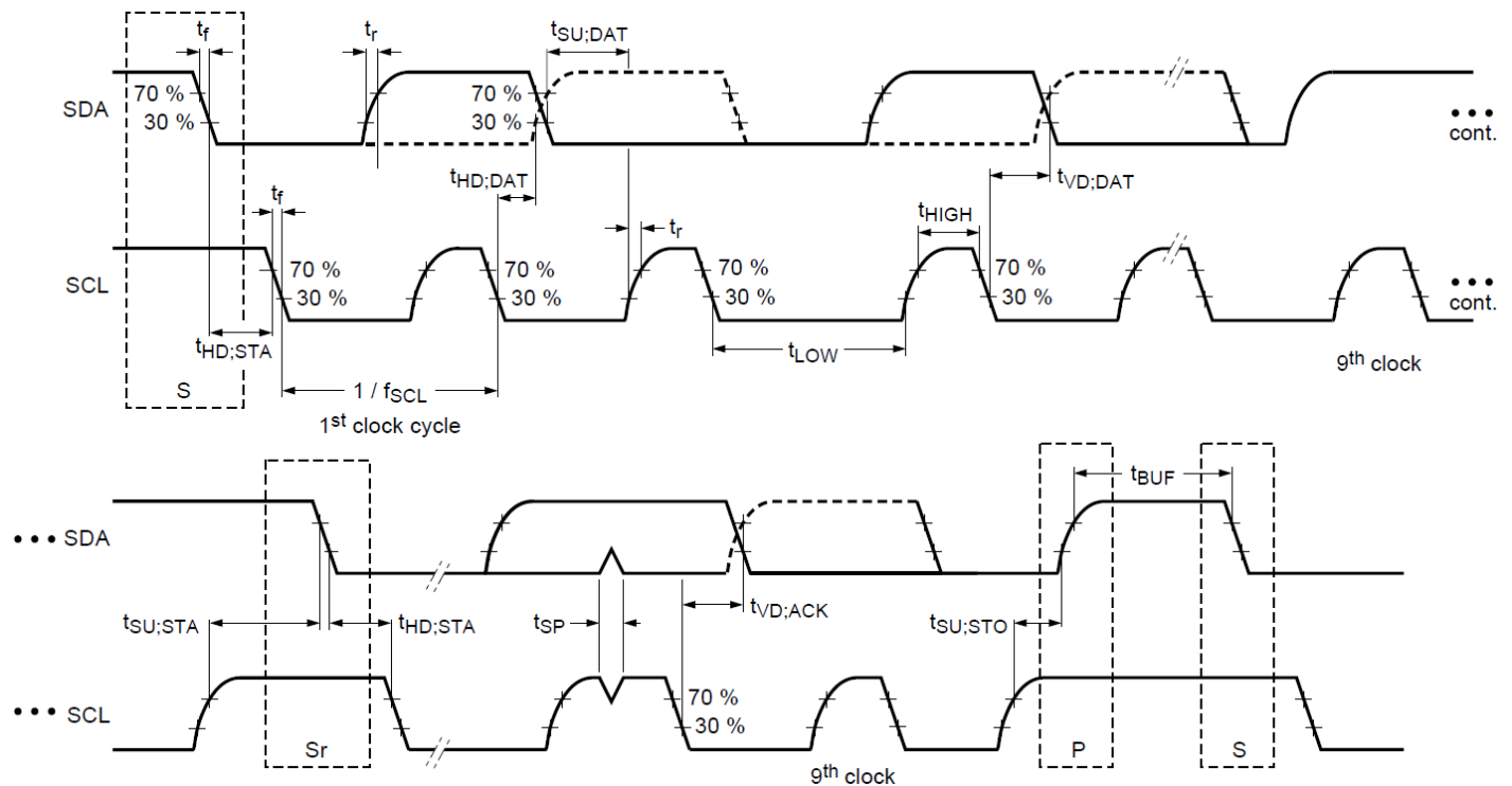
Figure 3: I2C Timing
