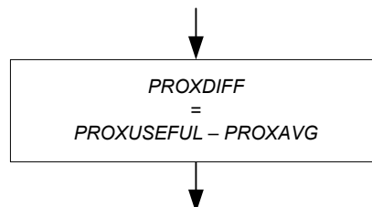
Figure 16: PROXDIFF Update
