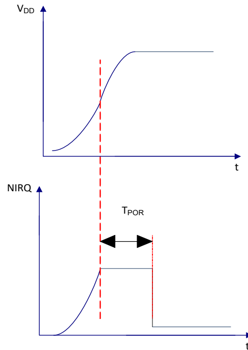
Figure 21: Power-up vs. NIRQ
