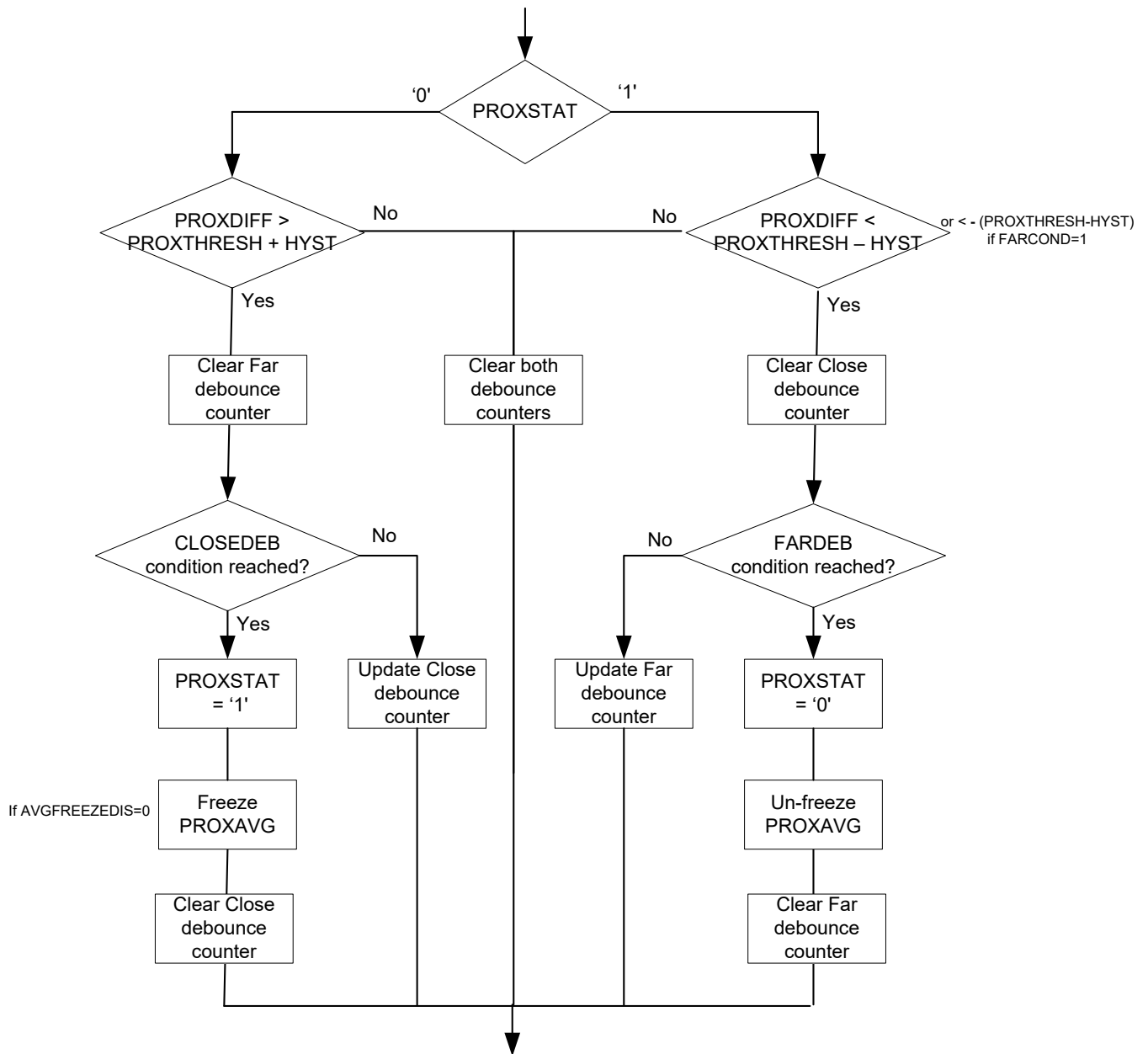
Figure 17: PROXSTAT Update
