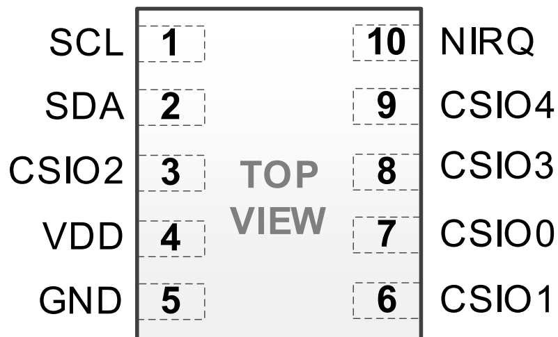
Figure 1: Pin Diagram
