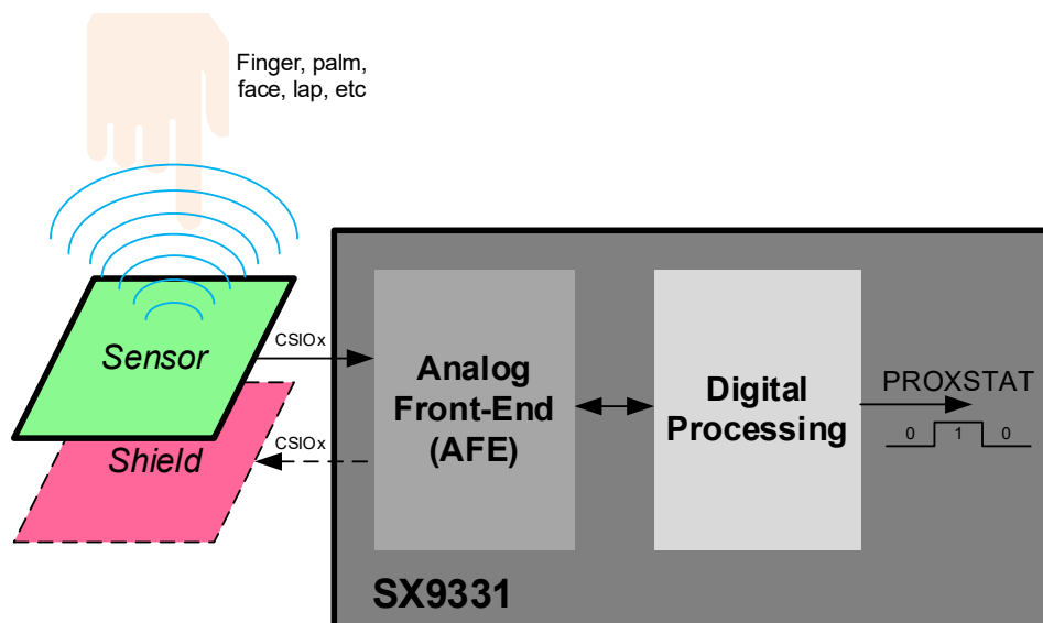
Figure 4: Proximity Sensing Interface Overview
