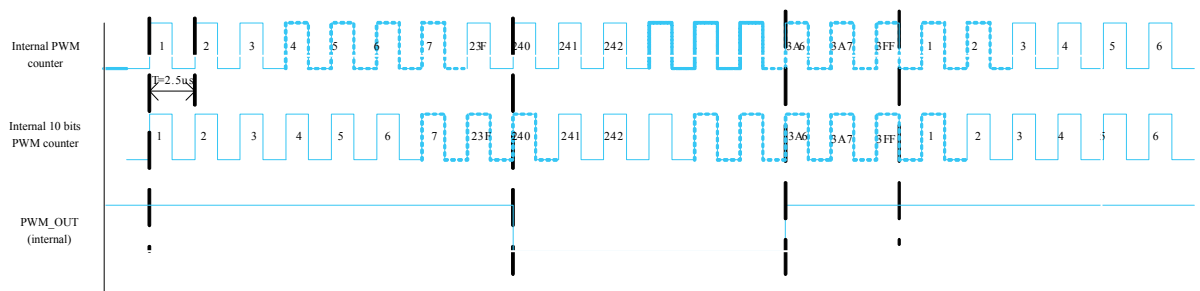
Figure 16. Resulting waveform 4
