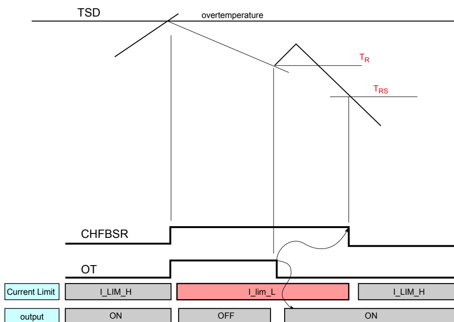
Figure 6. Thermal shutdown
