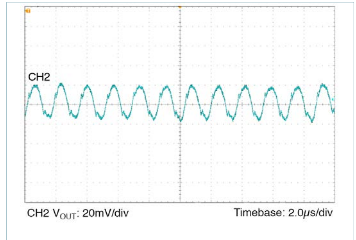
Figure 11 — Output ripple 12V IN 5.0V OUT at 15A; C_{OUT} = 8 \times 47\mu F
