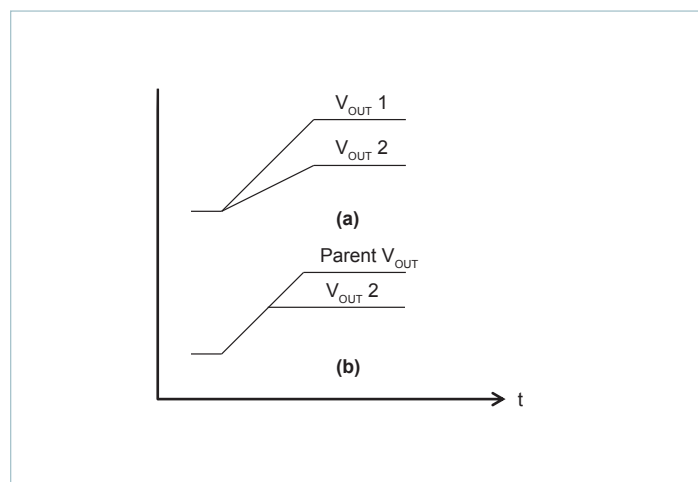
Figure 18 — PI34xx-00 tracking methods
