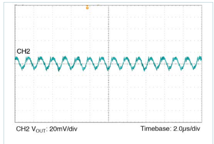
Figure 12 — Output ripple 12V IN 5.0V OUT at 7.0A; C_{OUT} = 8 \times 47\mu F
