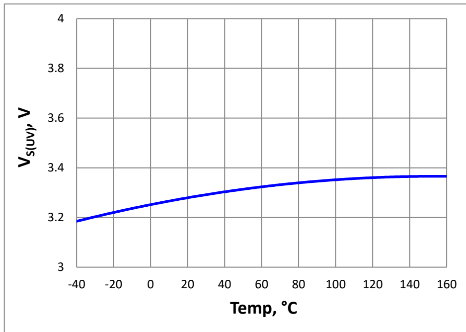
Figure 17. Undervoltage Shutdown V_{S(UV)} = f(T_J)
