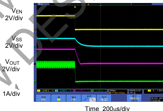
Enable Turn off Characteristic ( V_{IN}=12\text{V} , V_{EN}=3.3\text{V} , V_{OUT}=3.3\text{V} , I_L=2\text{A} )
