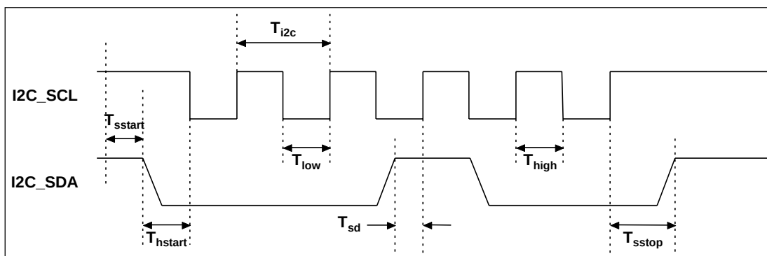
Figure 16: Interface Timings – I²C Fast Speed Mode
