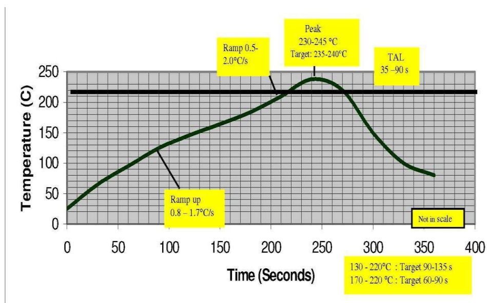
Figure 9: Reflow Diagram
