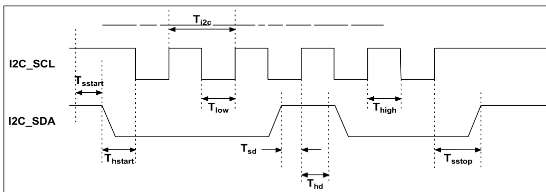
Figure 17: Interface Timings – I²C High Speed Mode
