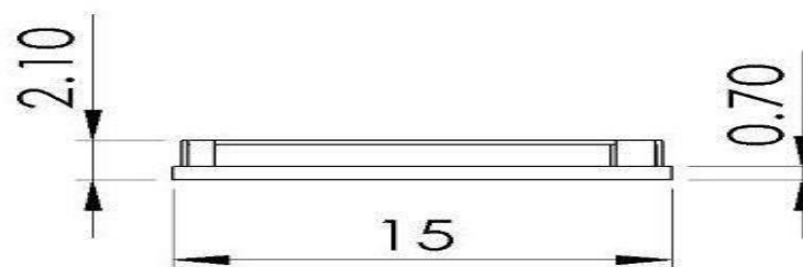
Figure 4: Package Dimensions of Module without Antenna
