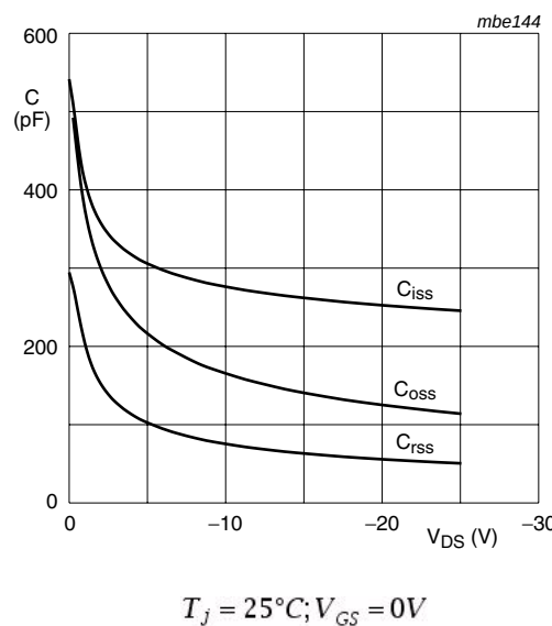
Fig 6. Capacitance as a function of drain-source voltage; P-channel; typical values
