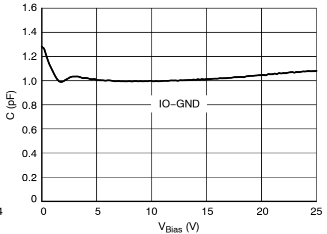
Figure 2. CV Characteristics
