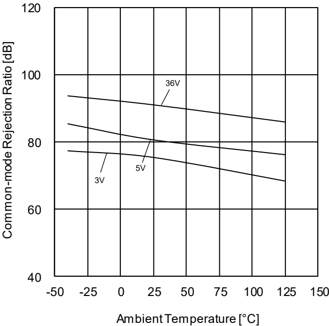
Figure 57. Common-mode Rejection Ratio vs Ambient Temperature
