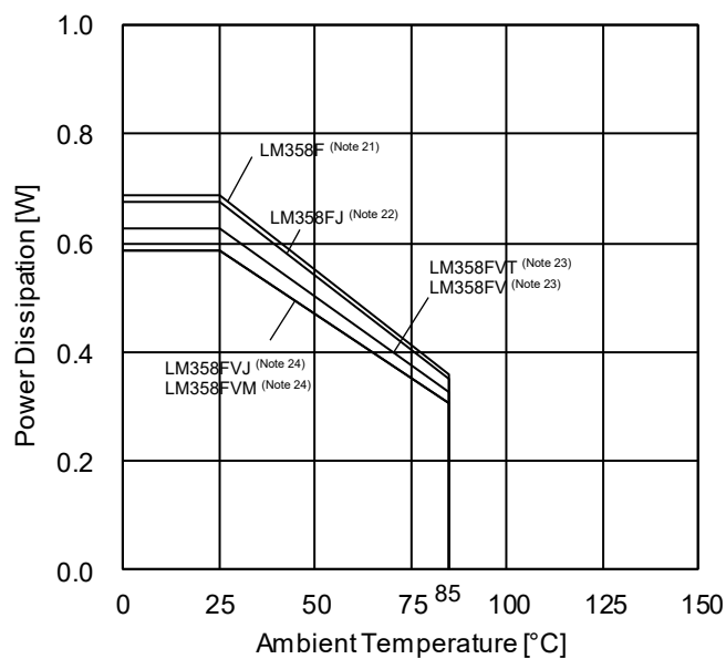
(c) LM358xxx *1
