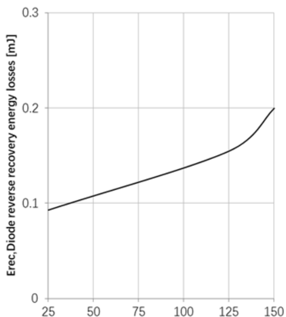
Fig21. Typical diode reverse recovery energy losses as a fuction of Junction temperature (inductive load, I_f=40A , V_{rr}=400V )
