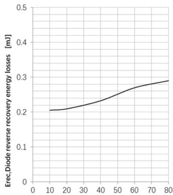
Fig22. Typical diode reverse recovery energy losses as a fuction of collect current (inductive load, T_{vj}=150^{\circ}C , V_{rr}=400V )
