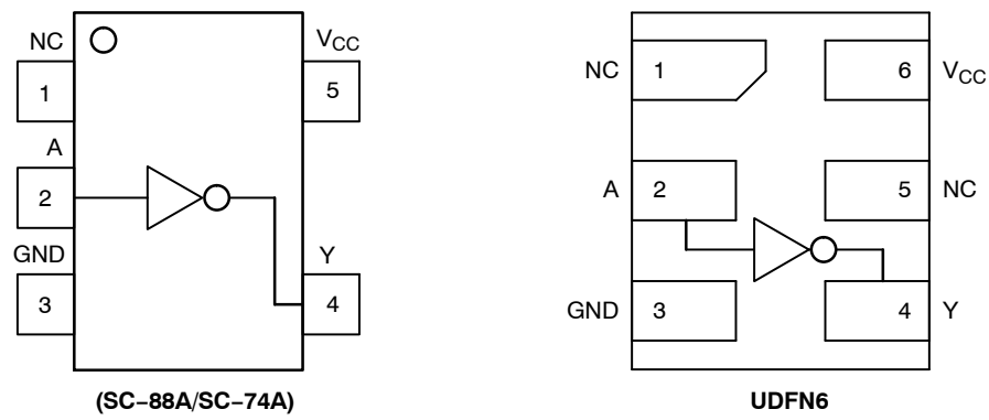
Figure 2. Pinout (Top View)
