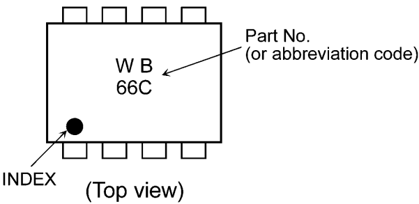
TC7WB66CFK
