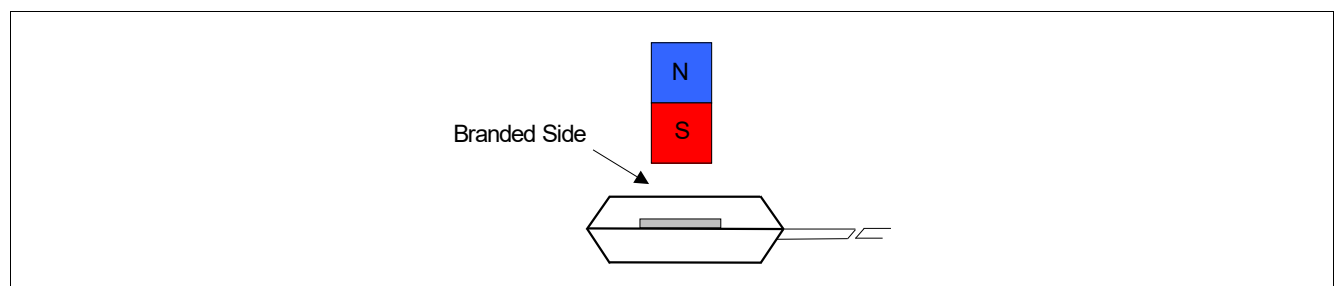
Figure 9 Definition of magnetic field direction T092S-3-1, T092S-3-2
