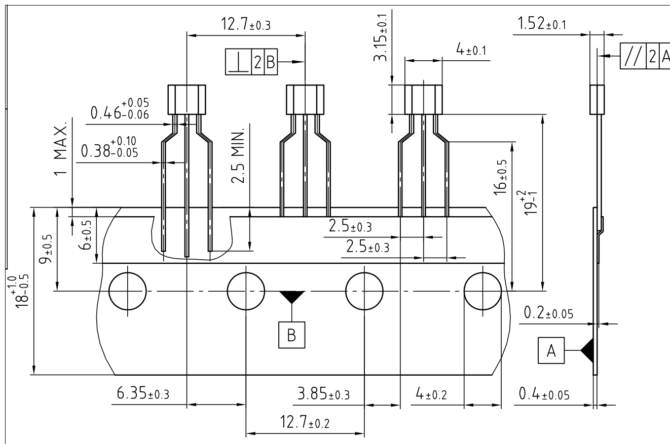
Figure 12 Packing information
