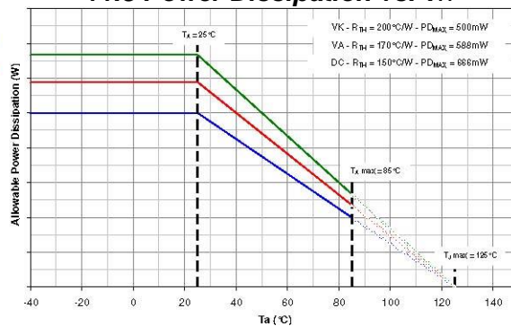
11.8 Power Dissipation vs. T_A
