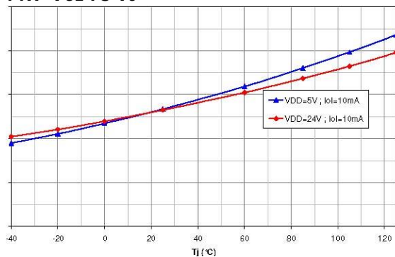
11.7 V_{OL} vs T_J
