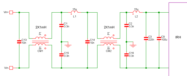
Figure 7. Conducted Emissions Test Circuit
