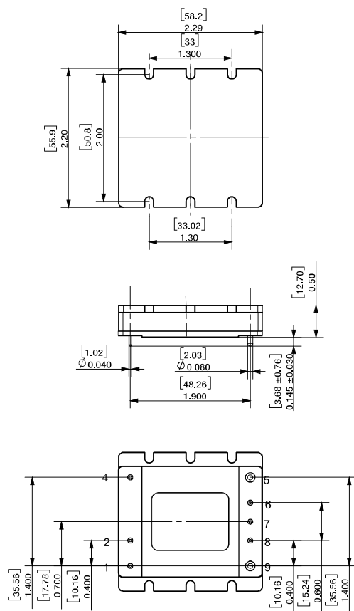
SLOTTED / FLANGED BASEPLATE
