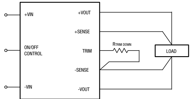
Figure 8 Trim Connections to Decrease Output Voltage
