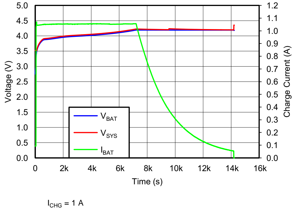
Figure 16. bq24250 Charge Profile while Charging a 2700-mAh Battery at a 1A Charge Rate
