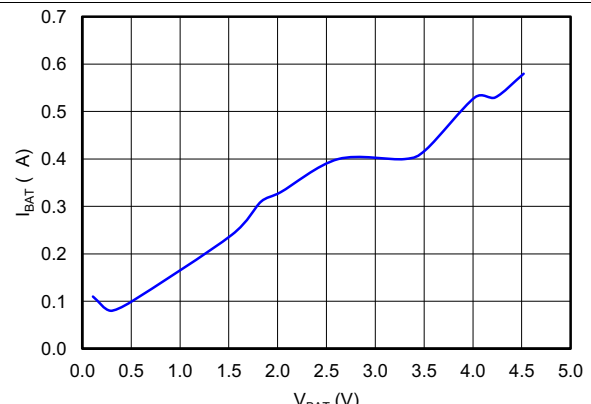
Figure 8. BAT IQ, SYSOFF = 1
