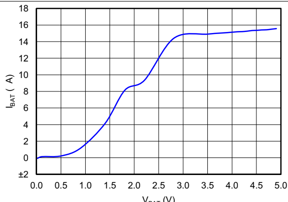
Figure 7. BAT IQ, SYSOFF = 0
