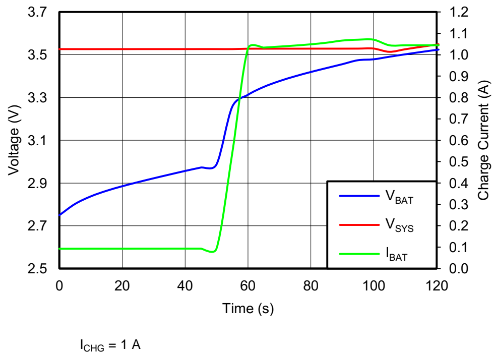
Figure 17. bq24250 Charge Profile While Charging a 2700-mAh Battery at a 1A Charge During Precharge
