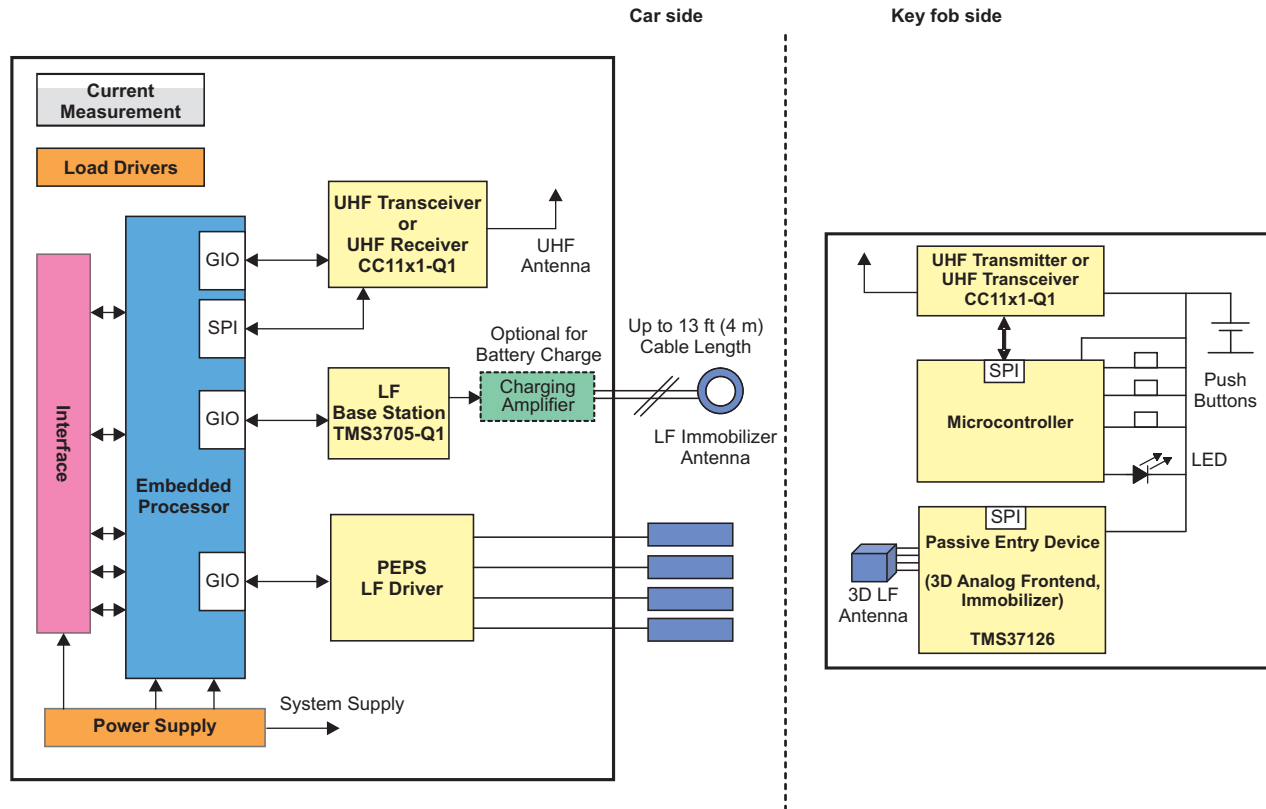
Figure 1. Application Diagram
