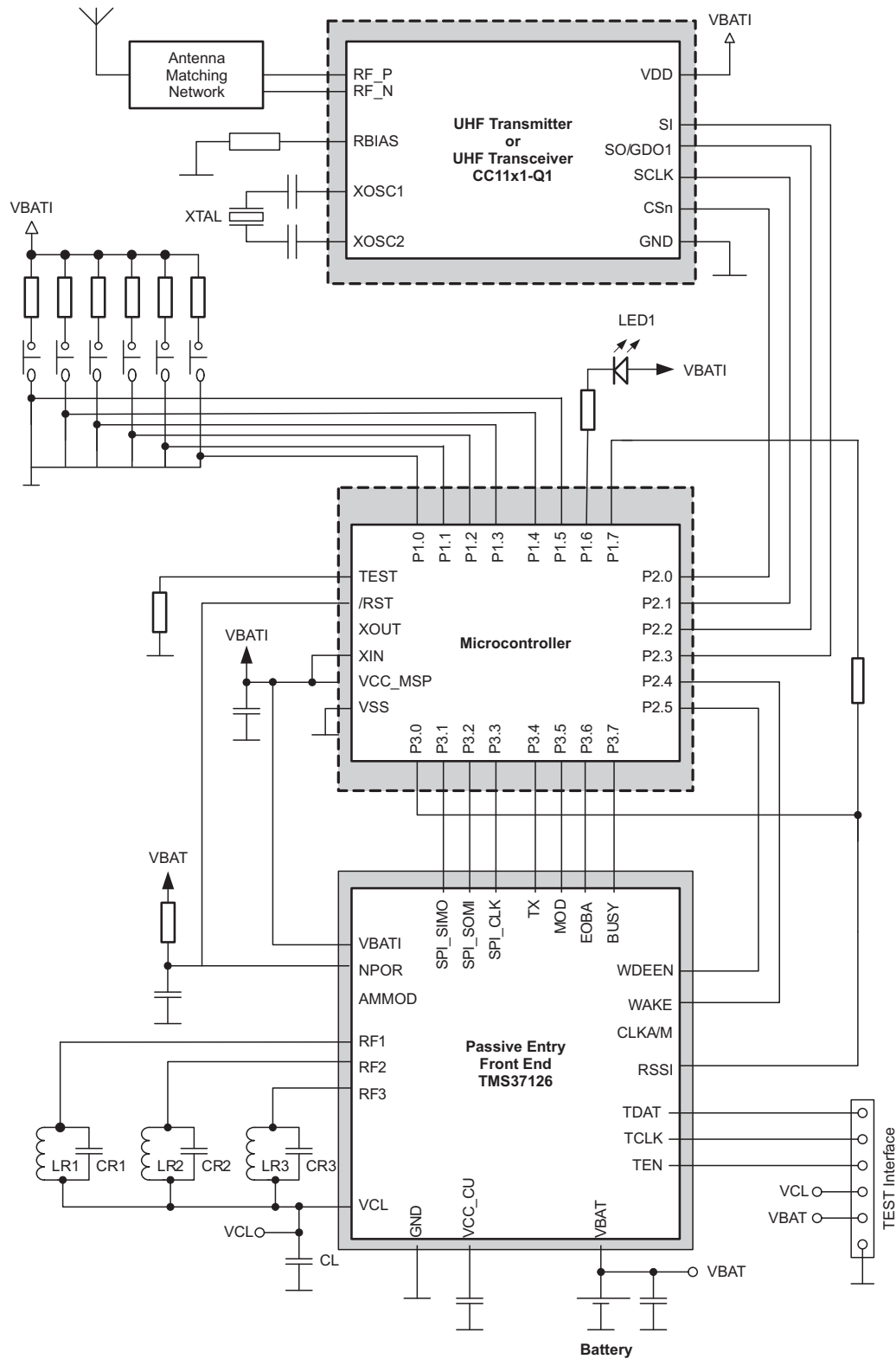
Figure 2. Application Schematic
