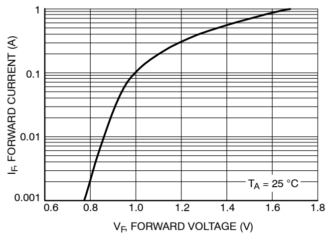
Figure 10. Forward Voltage
