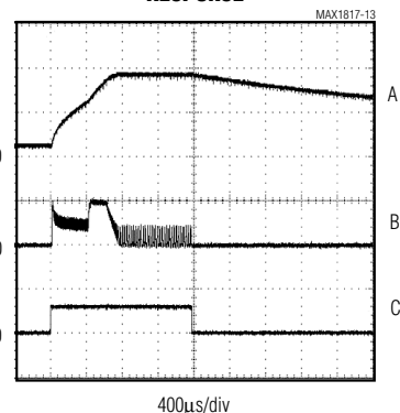
LCD OUTPUT TURN-ON/TURN-OFF RESPONSE
